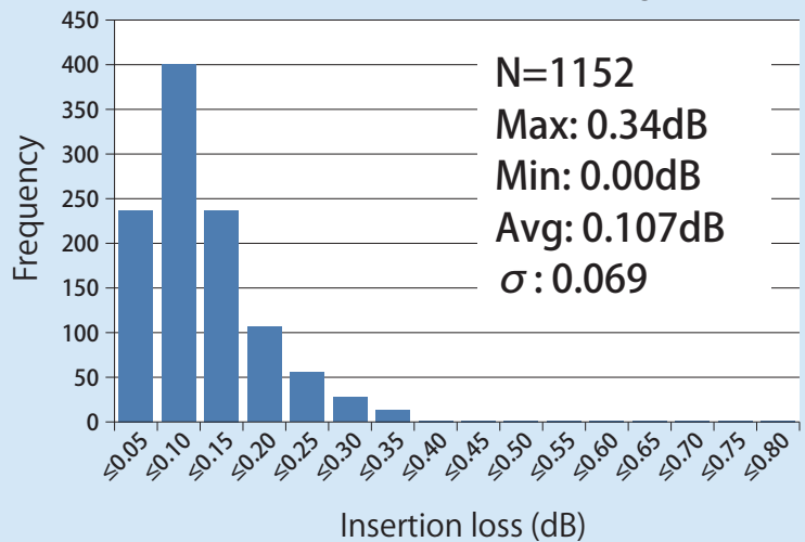
Insertion loss @1310nm for MT12SM-Low Loss Pre-angled
